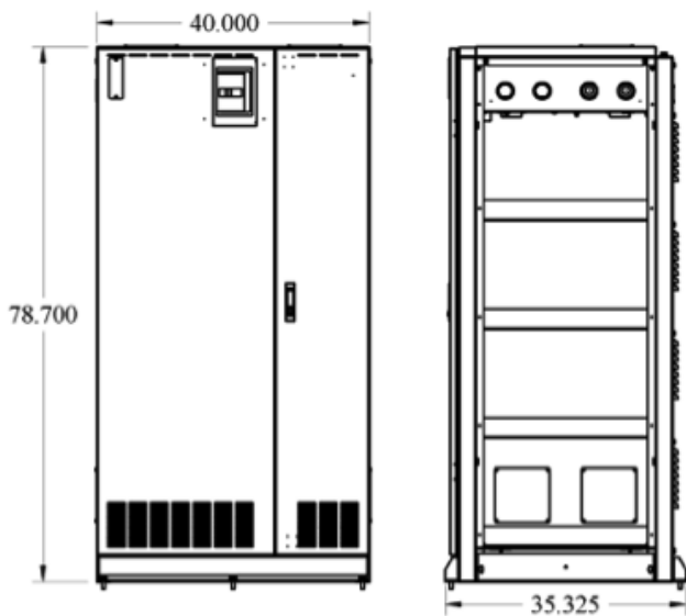
Front and side view and measurements, no side panels
