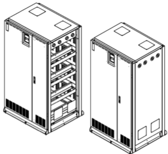
Isometric view with and without side panels
