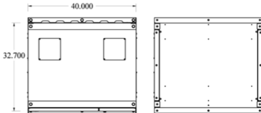
Top and bottom view
